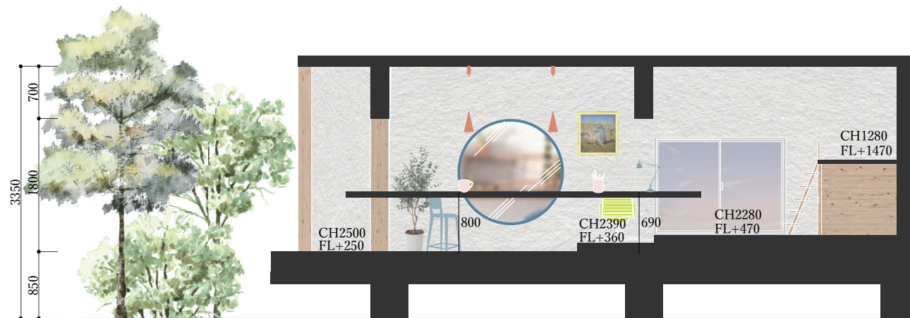
Section: S=1/50
